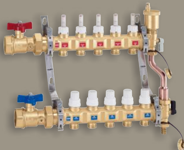
Pre-assembled, 5-way S1 manifold distribution system
